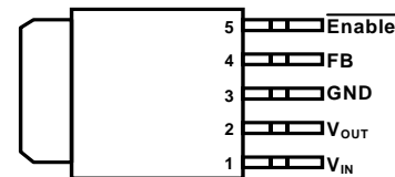
A307-ADJ TO-252 (Top View)
